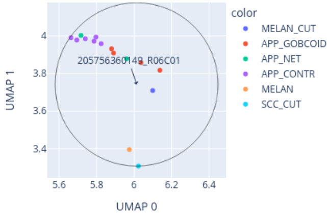
Close-up of UMAP for 205756360149_R06C01 reference: AllIDATv2_20210804_HPAP_Sarc.xlsx (19967 cases), 0 CpGs
