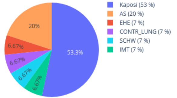
Neighbors in UMAP for 206084850022_R05C01 reference: AllIDATv2_20210804_HPAP_Sarc.xlsx (19967 cases), 0 CpGs
