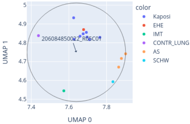
Close-up of UMAP for 206084850022_R05C01 reference: AllIDATv2_20210804_HPAP_Sarc.xlsx (19967 cases), 0 CpGs
