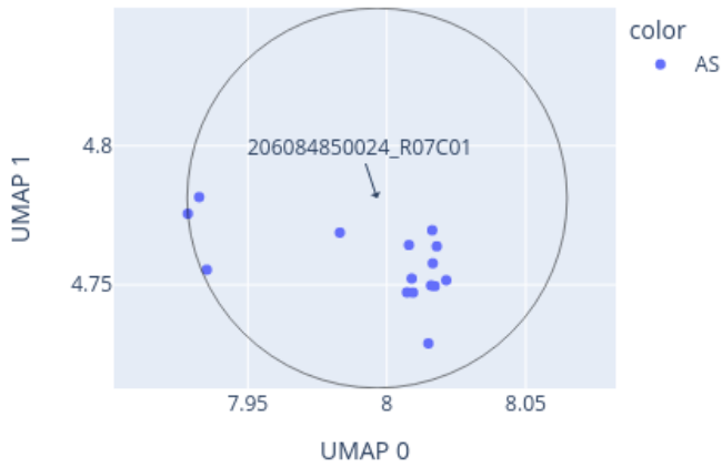
Close-up of UMAP for 206084850024_R07C01 reference: AllIDATv2_20210804_HPAP_Sarc.xlsx (19967 cases), 0 CpGs
