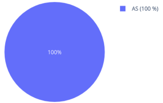
Neighbors in UMAP for 206084850024_R07C01 reference: AllIDATv2_20210804_HPAP_Sarc.xlsx (19967 cases), 0 CpGs
