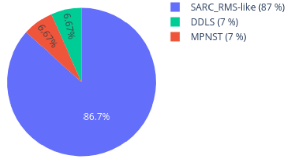
Neighbors in UMAP for 206095950017_R02C01 reference: AllIDATv2_20210804_HPAP_Sarc.xlsx (19967 cases), 0 CpGs
