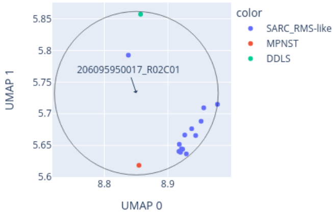
Close-up of UMAP for 206095950017_R02C01 reference: AllIDATv2_20210804_HPAP_Sarc.xlsx (19967 cases), 0 CpGs
