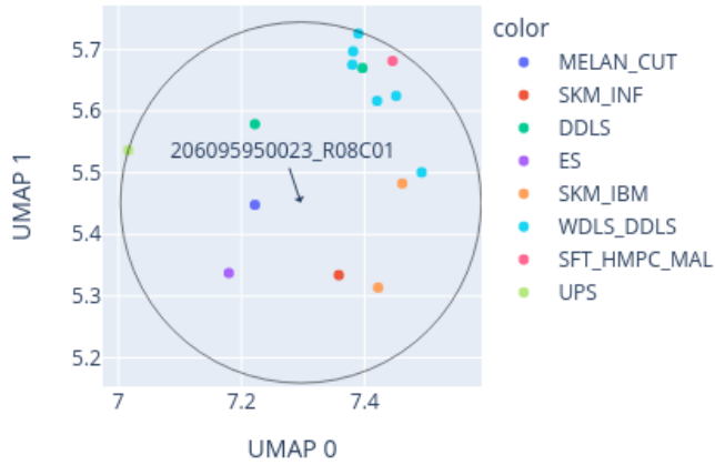
Close-up of UMAP for 206095950023_R08C01 reference: AllIDATv2_20210804_HPAP_Sarc.xlsx (19967 cases), 0 CpGs
