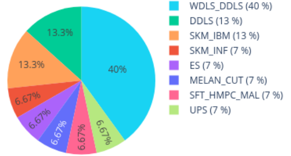
Neighbors in UMAP for 206095950023_R08C01 reference: AllIDATv2_20210804_HPAP_Sarc.xlsx (19967 cases), 0 CpGs
