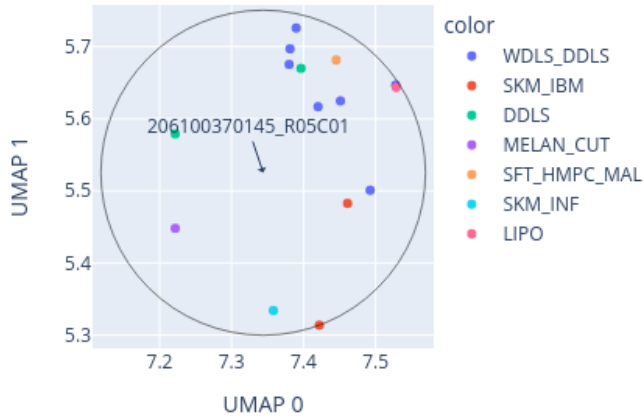
Close-up of UMAP for 206100370145_R05C01 reference: AllIDATv2_20210804_HPAP_Sarc.xlsx (19967 cases), 0 CpGs
