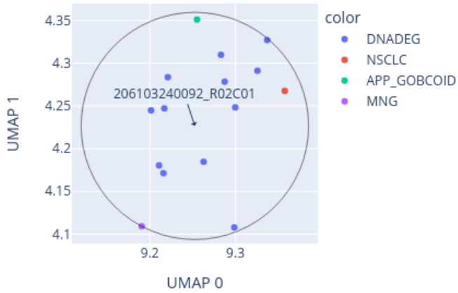
Close-up of UMAP for 206103240092_R02C01 reference: AllIDATv2_20210804_HPAP_Sarc.xlsx (19967 cases), 0 CpGs
