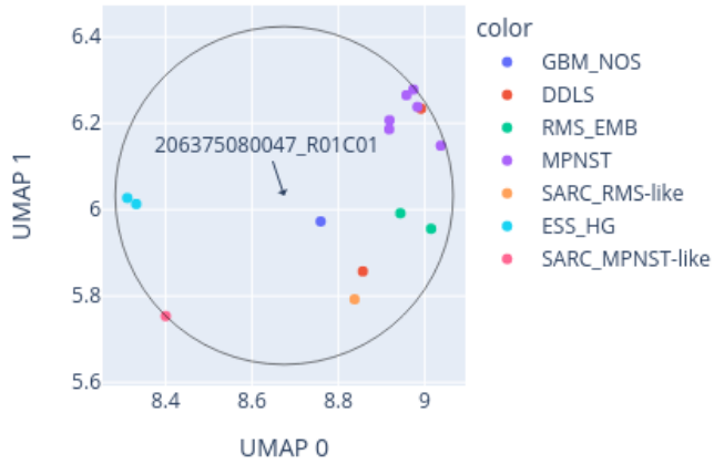
Close-up of UMAP for 206375080047_R01C01 reference: AllIDATv2_20210804_HPAP_Sarc.xlsx (19967 cases), 0 CpGs
