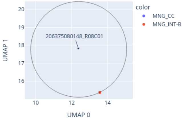
Close-up of UMAP for 206375080148_R08C01 reference: AllIDATv2_20210804_HPAP_Sarc.xlsx (19967 cases), 0 CpGs
