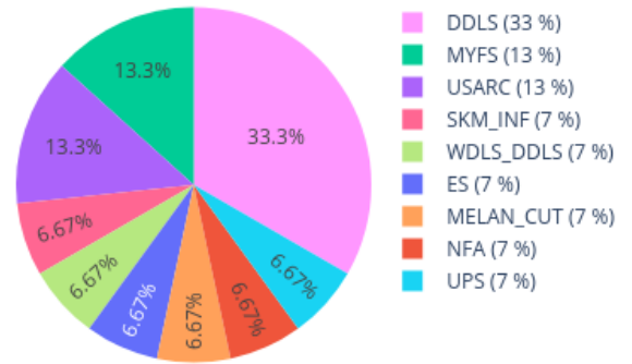
Neighbors in UMAP for 206382220019_R08C01 reference: AllIDATv2_20210804_HPAP_Sarc.xlsx (19967 cases), 0 CpGs
