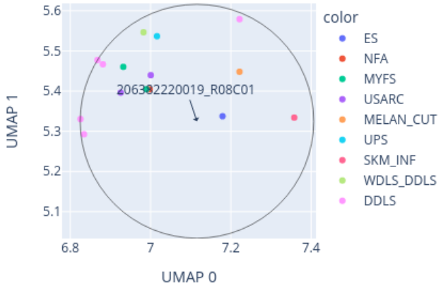
Close-up of UMAP for 206382220019_R08C01 reference: AllIDATv2_20210804_HPAP_Sarc.xlsx (19967 cases), 0 CpGs
