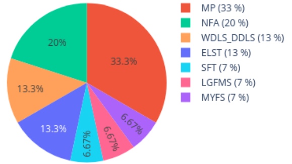
Neighbors in UMAP for 206382220028_R01C01 reference: AllIDATv2_20210804_HPAP_Sarc.xlsx (19967 cases), 0 CpGs
