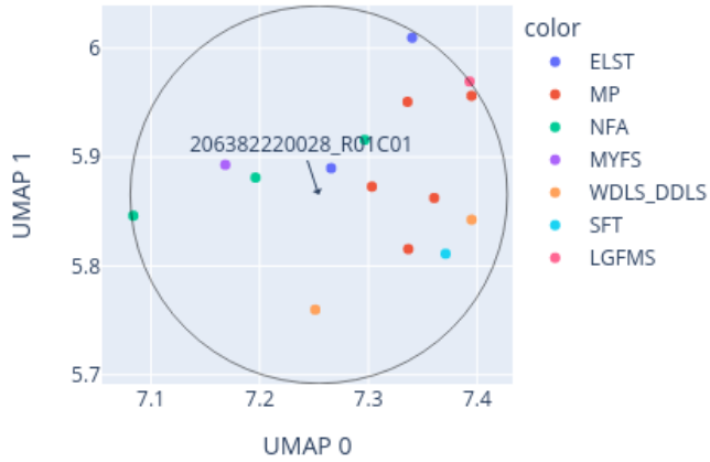
Close-up of UMAP for 206382220028_R01C01 reference: AllIDATv2_20210804_HPAP_Sarc.xlsx (19967 cases), 0 CpGs
