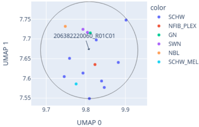
Close-up of UMAP for 206382220060_R01C01 reference: AllIDATv2_20210804_HPAP_Sarc.xlsx (19967 cases), 0 CpGs
