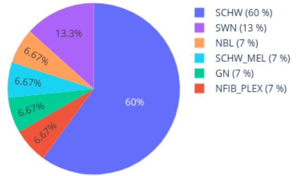
Neighbors in UMAP for 206382220060_R01C01 reference: AllIDATv2_20210804_HPAP_Sarc.xlsx (19967 cases), 0 CpGs
