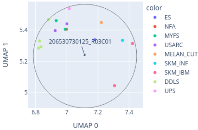
Close-up of UMAP for 206530730125_R03C01 reference: AllIDATv2_20210804_HPAP_Sarc.xlsx (19967 cases), 0 CpGs
