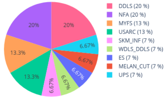
Neighbors in UMAP for 206535560078_R01C01 reference: AllIDATv2_20210804_HPAP_Sarc.xlsx (19967 cases), 0 CpGs
