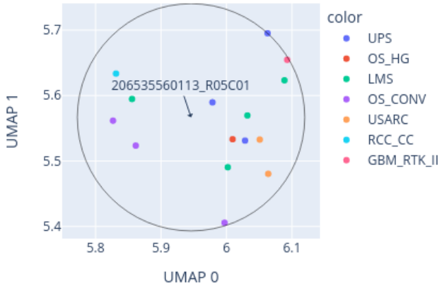
Close-up of UMAP for 206535560113_R05C01 reference: AllIDATv2_20210804_HPAP_Sarc.xlsx (19967 cases), 0 CpGs
