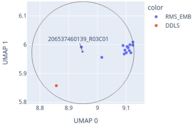
Close-up of UMAP for 206537460139_R03C01 reference: AllIDATv2_20210804_HPAP_Sarc.xlsx (19967 cases), 0 CpGs
