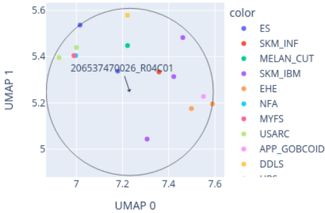
Close-up of UMAP for 206537470026_R04C01 reference: AllIDATv2_20210804_HPAP_Sarc.xlsx (19967 cases), 0 CpGs
