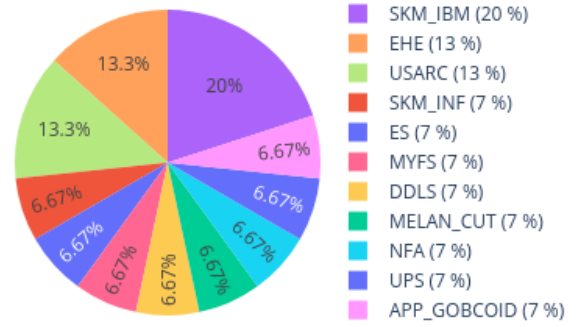
Neighbors in UMAP for 206537470026_R04C01 reference: AllIDATv2_20210804_HPAP_Sarc.xlsx (19967 cases), 0 CpGs
