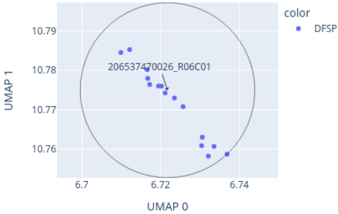
Close-up of UMAP for 206537470026_R06C01 reference: AllIDATv2_20210804_HPAP_Sarc.xlsx (19967 cases), 0 CpGs
