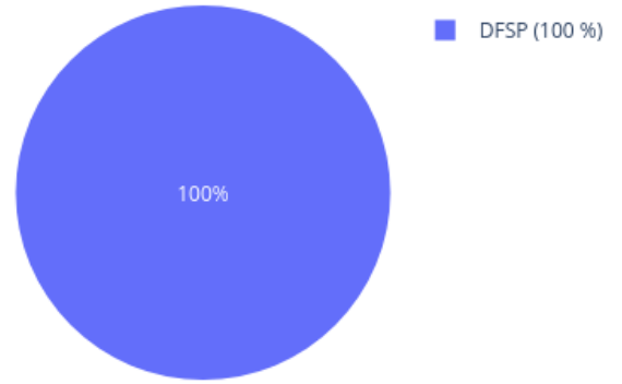
Neighbors in UMAP for 206537470026_R06C01 reference: AllIDATv2_20210804_HPAP_Sarc.xlsx (19967 cases), 0 CpGs
