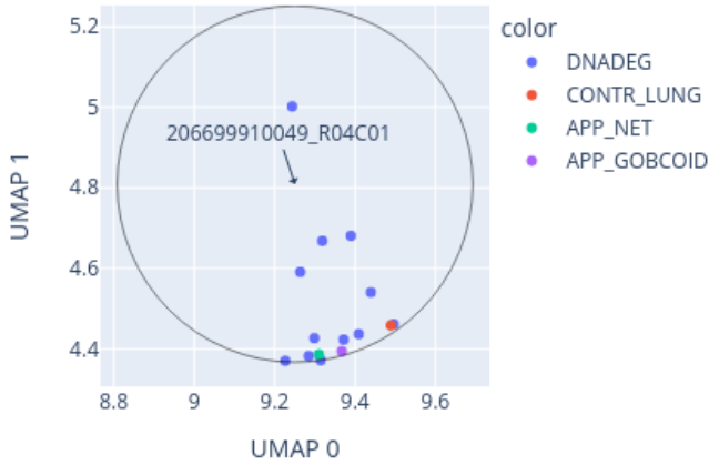
Close-up of UMAP for 206699910049_R04C01 reference: AllIDATv2_20210804_HPAP_Sarc.xlsx (19967 cases), 0 CpGs
