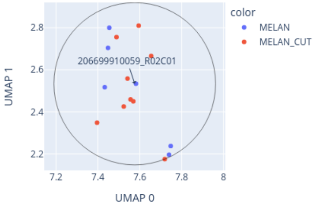
Close-up of UMAP for 206699910059_R02C01 reference: AllIDATv2_20210804_HPAP_Sarc.xlsx (19967 cases), 0 CpGs
