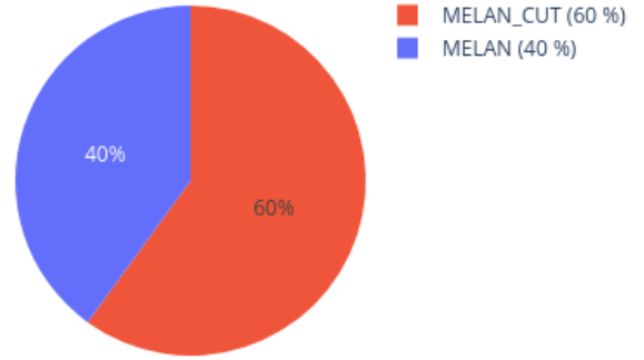
Neighbors in UMAP for 206699910059_R02C01 reference: AllIDATv2_20210804_HPAP_Sarc.xlsx (19967 cases), 0 CpGs
