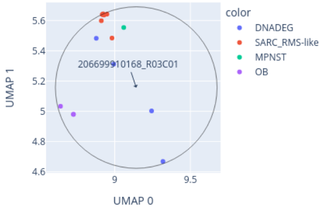
Close-up of UMAP for 206699910168_R03C01 reference: AllIDATv2_20210804_HPAP_Sarc.xlsx (19967 cases), 0 CpGs
