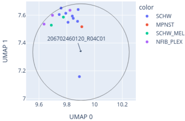
Close-up of UMAP for 206702460120_R04C01 reference: AllIDATv2_20210804_HPAP_Sarc.xlsx (19967 cases), 0 CpGs
