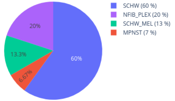
Neighbors in UMAP for 206702460120_R04C01 reference: AllIDATv2_20210804_HPAP_Sarc.xlsx (19967 cases), 0 CpGs
