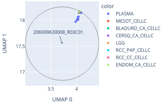
Close-up of UMAP for 206909630008_R03C01 reference: AllIDATv2_20210804_HPAP_Sarc.xlsx (19967 cases), 0 CpGs
