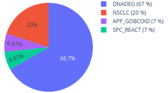
Neighbors in UMAP for 206909630042_R04C01 reference: AllIDATv2_20210804_HPAP_Sarc.xlsx (19967 cases), 0 CpGs
