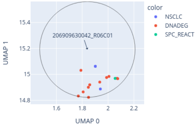
Close-up of UMAP for 206909630042_R06C01 reference: AllIDATv2_20210804_HPAP_Sarc.xlsx (19967 cases), 0 CpGs
