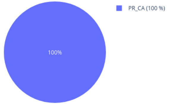
Neighbors in UMAP for 206909630051_R01C01 reference: AllIDATv2_20210804_HPAP_Sarc.xlsx (19967 cases), 0 CpGs
