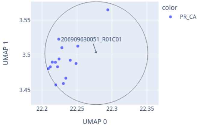
Close-up of UMAP for 206909630051_R01C01 reference: AllIDATv2_20210804_HPAP_Sarc.xlsx (19967 cases), 0 CpGs
