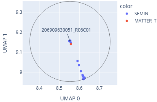
Close-up of UMAP for 206909630051_R06C01 reference: AllIDATv2_20210804_HPAP_Sarc.xlsx (19967 cases), 0 CpGs
