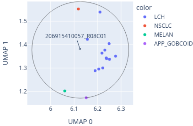
Close-up of UMAP for 206915410057_R08C01 reference: AllIDATv2_20210804_HPAP_Sarc.xlsx (19967 cases), 0 CpGs
