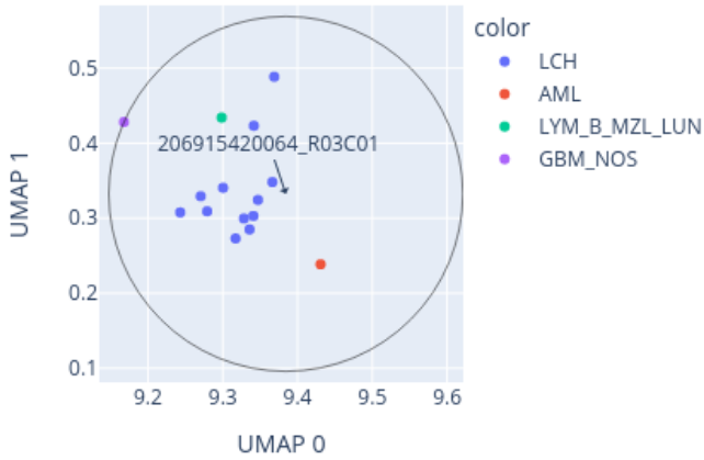
Close-up of UMAP for 206915420064_R03C01 reference: AllIDATv2_20210804_HPAP_Sarc.xlsx (19967 cases), 0 CpGs
