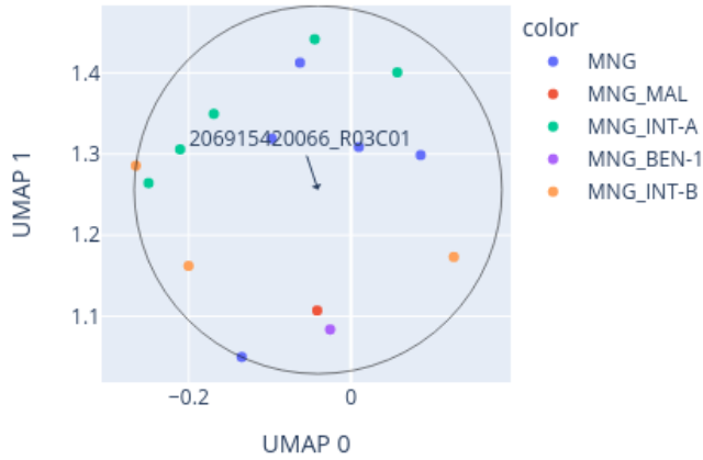
Close-up of UMAP for 206915420066_R03C01 reference: AllIDATv2_20210804_HPAP_Sarc.xlsx (19967 cases), 0 CpGs
