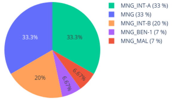
Neighbors in UMAP for 206915420066_R03C01 reference: AllIDATv2_20210804_HPAP_Sarc.xlsx (19967 cases), 0 CpGs
