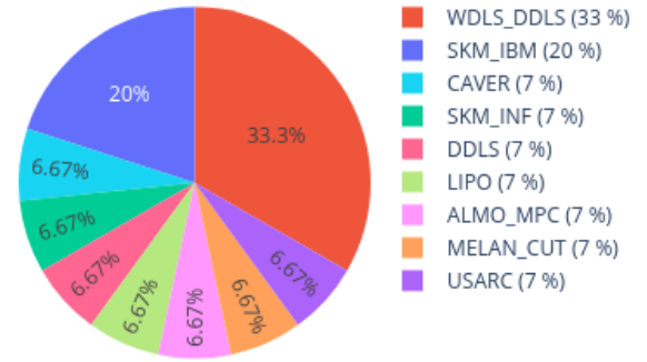
Neighbors in UMAP for 207019360011_R01C01 reference: AllIDATv2_20210804_HPAP_Sarc.xlsx (19967 cases), 0 CpGs
