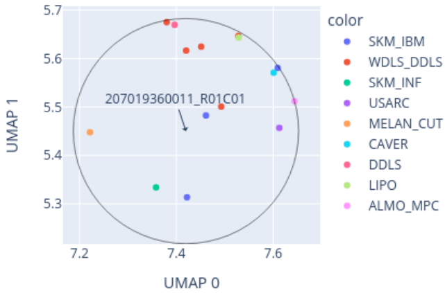
Close-up of UMAP for 207019360011_R01C01 reference: AllIDATv2_20210804_HPAP_Sarc.xlsx (19967 cases), 0 CpGs
