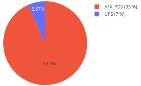
Neighbors in UMAP for 207019360042_R04C01 reference: AllIDATv2_20210804_HPAP_Sarc.xlsx (19967 cases), 0 CpGs
