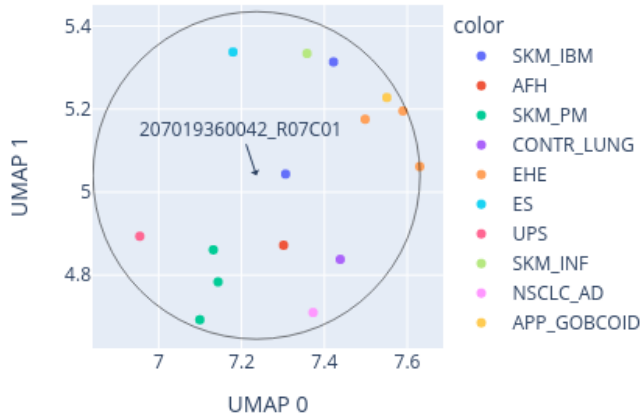
Close-up of UMAP for 207019360042_R07C01 reference: AllIDATv2_20210804_HPAP_Sarc.xlsx (19967 cases), 0 CpGs
