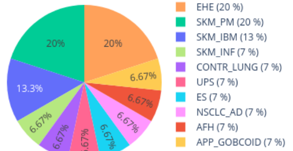
Neighbors in UMAP for 207019360042_R07C01 reference: AllIDATv2_20210804_HPAP_Sarc.xlsx (19967 cases), 0 CpGs
