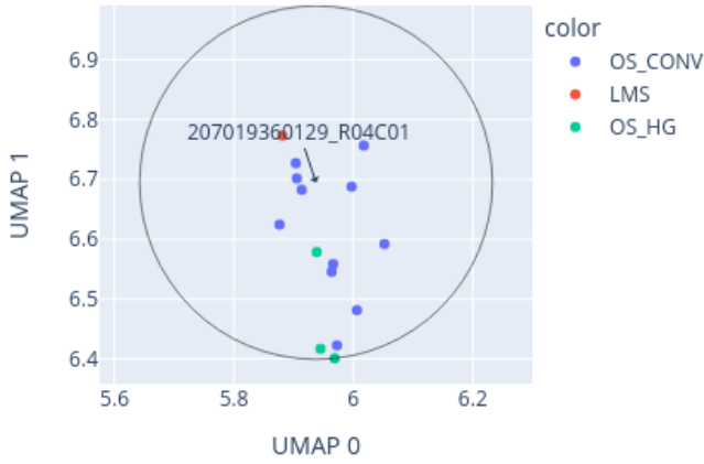
Close-up of UMAP for 207019360129_R04C01 reference: AllIDATv2_20210804_HPAP_Sarc.xlsx (19967 cases), 0 CpGs
