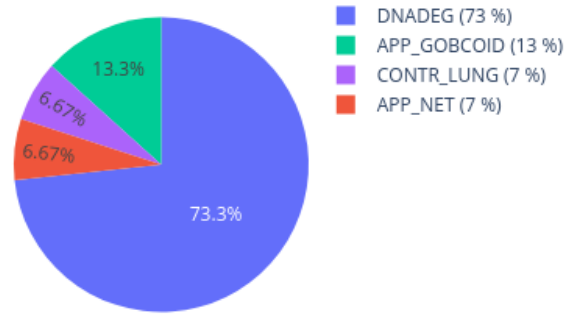
Neighbors in UMAP for 207019360144_R01C01 reference: AllIDATv2_20210804_HPAP_Sarc.xlsx (19967 cases), 0 CpGs
