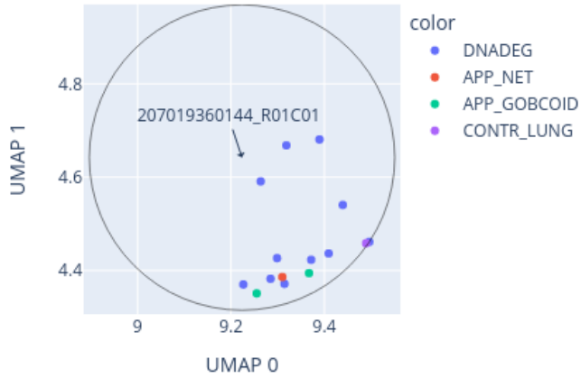
Close-up of UMAP for 207019360144_R01C01 reference: AllIDATv2_20210804_HPAP_Sarc.xlsx (19967 cases), 0 CpGs
