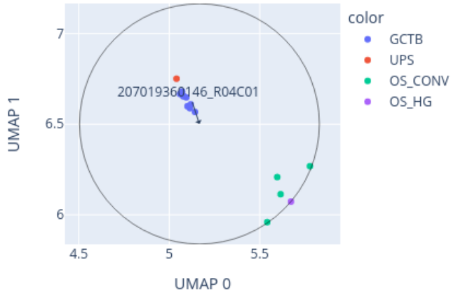
Close-up of UMAP for 207019360146_R04C01 reference: AllIDATv2_20210804_HPAP_Sarc.xlsx (19967 cases), 0 CpGs
