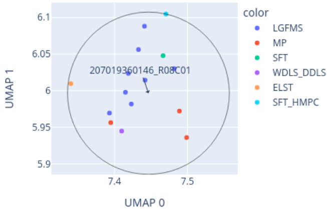
Close-up of UMAP for 207019360146_R08C01 reference: AllIDATv2_20210804_HPAP_Sarc.xlsx (19967 cases), 0 CpGs
