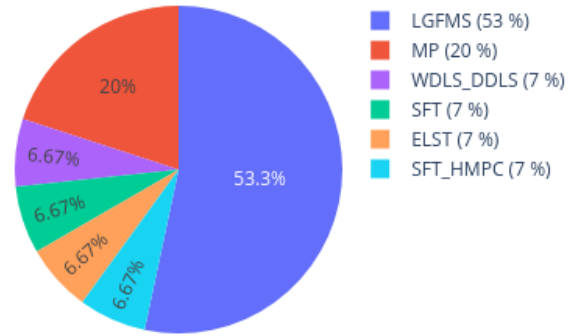
Neighbors in UMAP for 207019360146_R08C01 reference: AllIDATv2_20210804_HPAP_Sarc.xlsx (19967 cases), 0 CpGs
