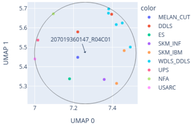
Close-up of UMAP for 207019360147_R04C01 reference: AllIDATv2_20210804_HPAP_Sarc.xlsx (19967 cases), 0 CpGs
