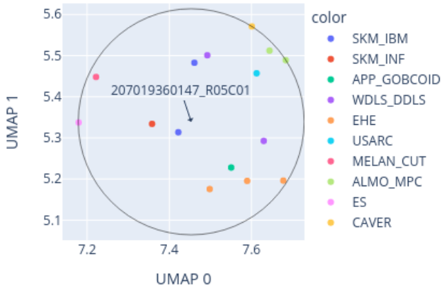
Close-up of UMAP for 207019360147_R05C01 reference: AllIDATv2_20210804_HPAP_Sarc.xlsx (19967 cases), 0 CpGs
