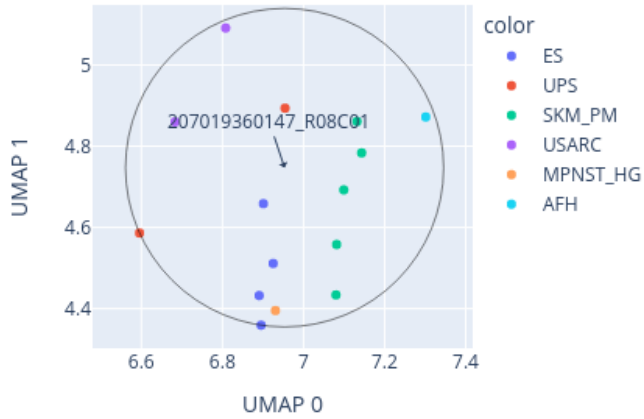
Close-up of UMAP for 207019360147_R08C01 reference: AllIDATv2_20210804_HPAP_Sarc.xlsx (19967 cases), 0 CpGs
