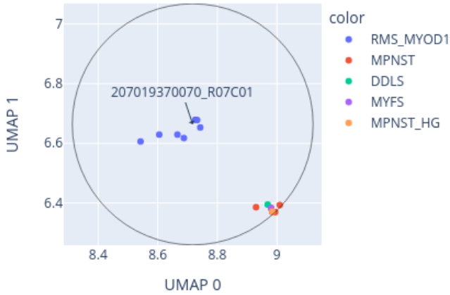
Close-up of UMAP for 207019370070_R07C01 reference: AllIDATv2_20210804_HPAP_Sarc.xlsx (19967 cases), 0 CpGs
