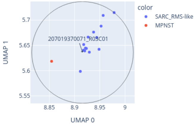
Close-up of UMAP for 207019370071_R03C01 reference: AllIDATv2_20210804_HPAP_Sarc.xlsx (19967 cases), 0 CpGs
