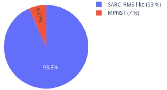
Neighbors in UMAP for 207019370071_R03C01 reference: AllIDATv2_20210804_HPAP_Sarc.xlsx (19967 cases), 0 CpGs
