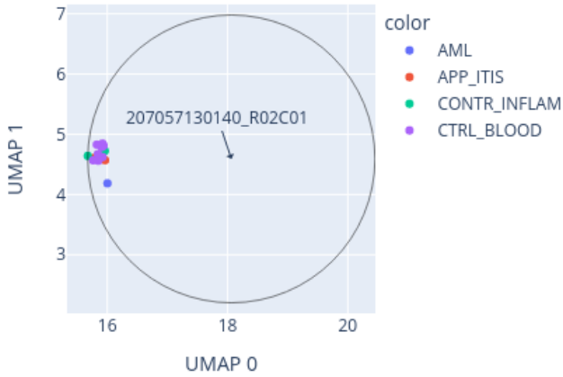
Close-up of UMAP for 207057130140_R02C01 reference: AllIDATv2_20210804_HPAP_Sarc.xlsx (19967 cases), 0 CpGs
