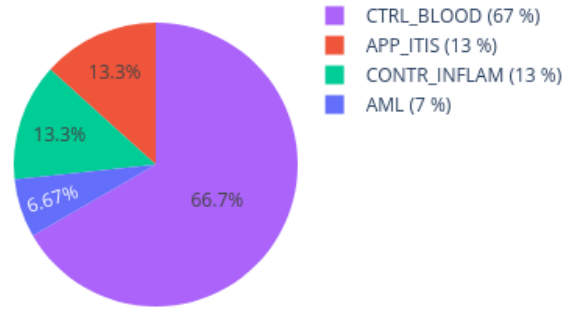
Neighbors in UMAP for 207057130140_R02C01 reference: AllIDATv2_20210804_HPAP_Sarc.xlsx (19967 cases), 0 CpGs
