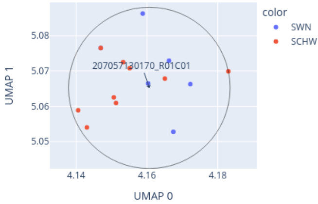
Close-up of UMAP for 207057130170_R01C01 reference: AllIDATv2_20210804_HPAP_Sarc.xlsx (19967 cases), 0 CpGs
