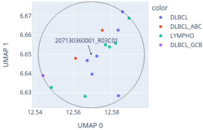
Close-up of UMAP for 207130360001_R03C01 reference: AllIDATv2_20210804_HPAP_Sarc.xlsx (19967 cases), 0 CpGs
