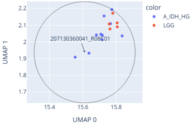
Close-up of UMAP for 207130360041_R08C01 reference: AllIDATv2_20210804_HPAP_Sarc.xlsx (19967 cases), 0 CpGs
