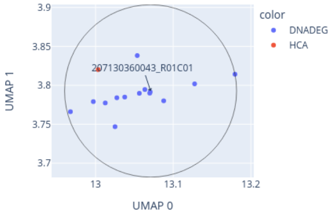
Close-up of UMAP for 207130360043_R01C01 reference: AllIDATv2_20210804_HPAP_Sarc.xlsx (19967 cases), 0 CpGs
