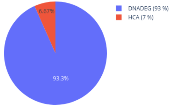
Neighbors in UMAP for 207130360043_R01C01 reference: AllIDATv2_20210804_HPAP_Sarc.xlsx (19967 cases), 0 CpGs
