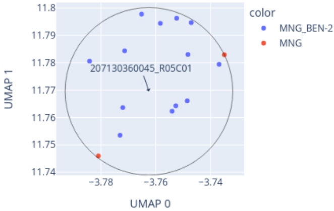
Close-up of UMAP for 207130360045_R05C01 reference: AllIDATv2_20210804_HPAP_Sarc.xlsx (19967 cases), 0 CpGs
