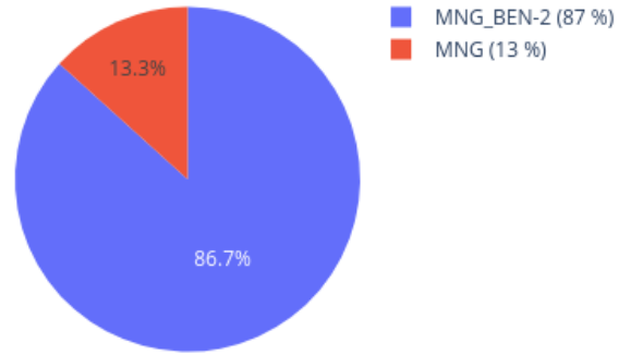
Neighbors in UMAP for 207130360045_R05C01 reference: AllIDATv2_20210804_HPAP_Sarc.xlsx (19967 cases), 0 CpGs
