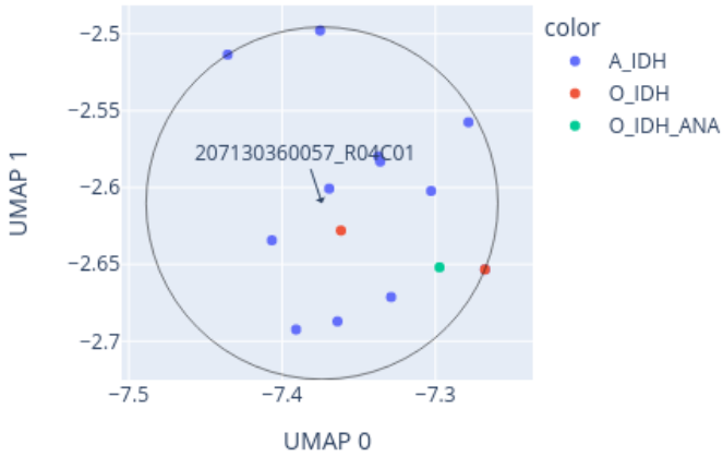
Close-up of UMAP for 207130360057_R04C01 reference: AllIDATv2_20210804_HPAP_Sarc.xlsx (19967 cases), 0 CpGs
