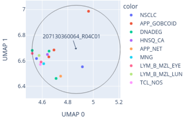
Close-up of UMAP for 207130360064_R04C01 reference: AllIDATv2_20210804_HPAP_Sarc.xlsx (19967 cases), 0 CpGs
