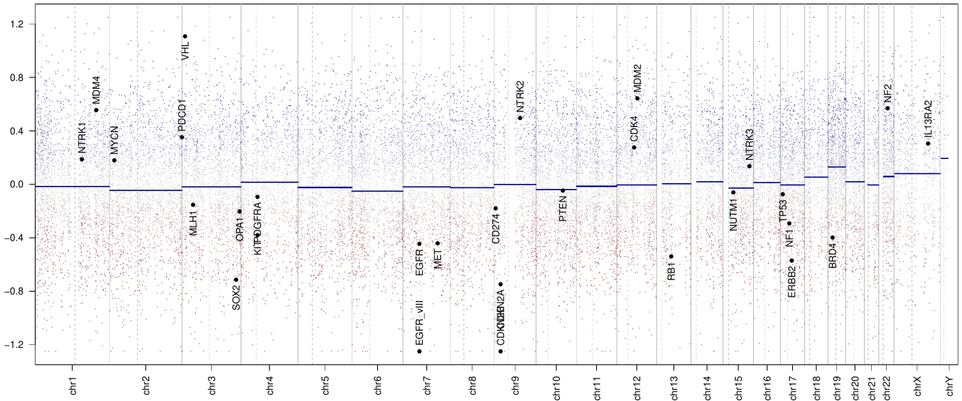
207130360064_R04C01
