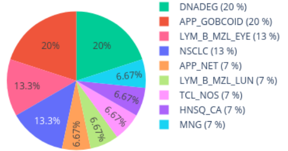
Neighbors in UMAP for 207130360064_R04C01 reference: AllIDATv2_20210804_HPAP_Sarc.xlsx (19967 cases), 0 CpGs
